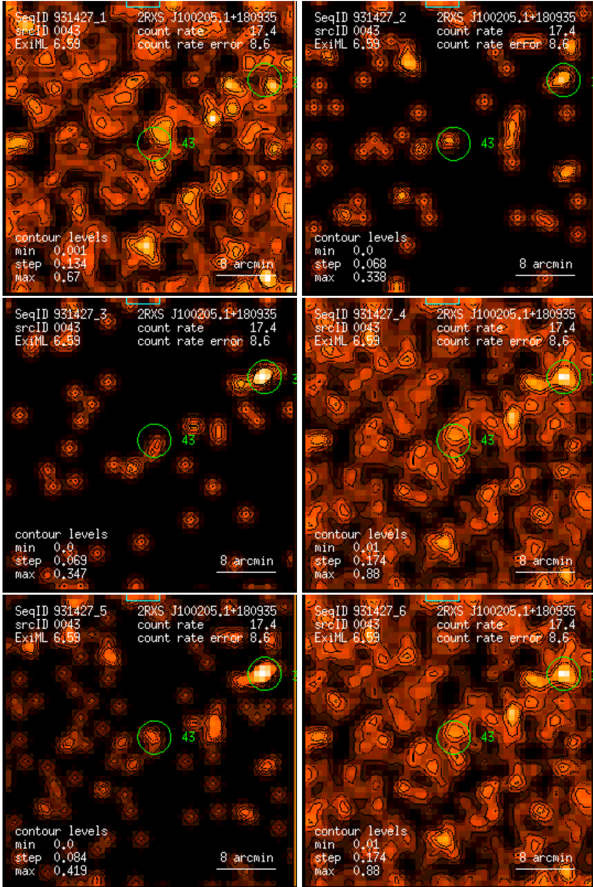
Figure 43: RASS 931427: detection 0043: band rate images, Gaussian filter: (1) PSPC channels 11 – 41, (2) 52 – 90, (3) 91 – 201, (4) 11 – 235, (5) 52 – 201, (6) 11 – 201. Broad band rates in counts/ks. Band rate contour levels in counts/ks/arcmin 2 .
