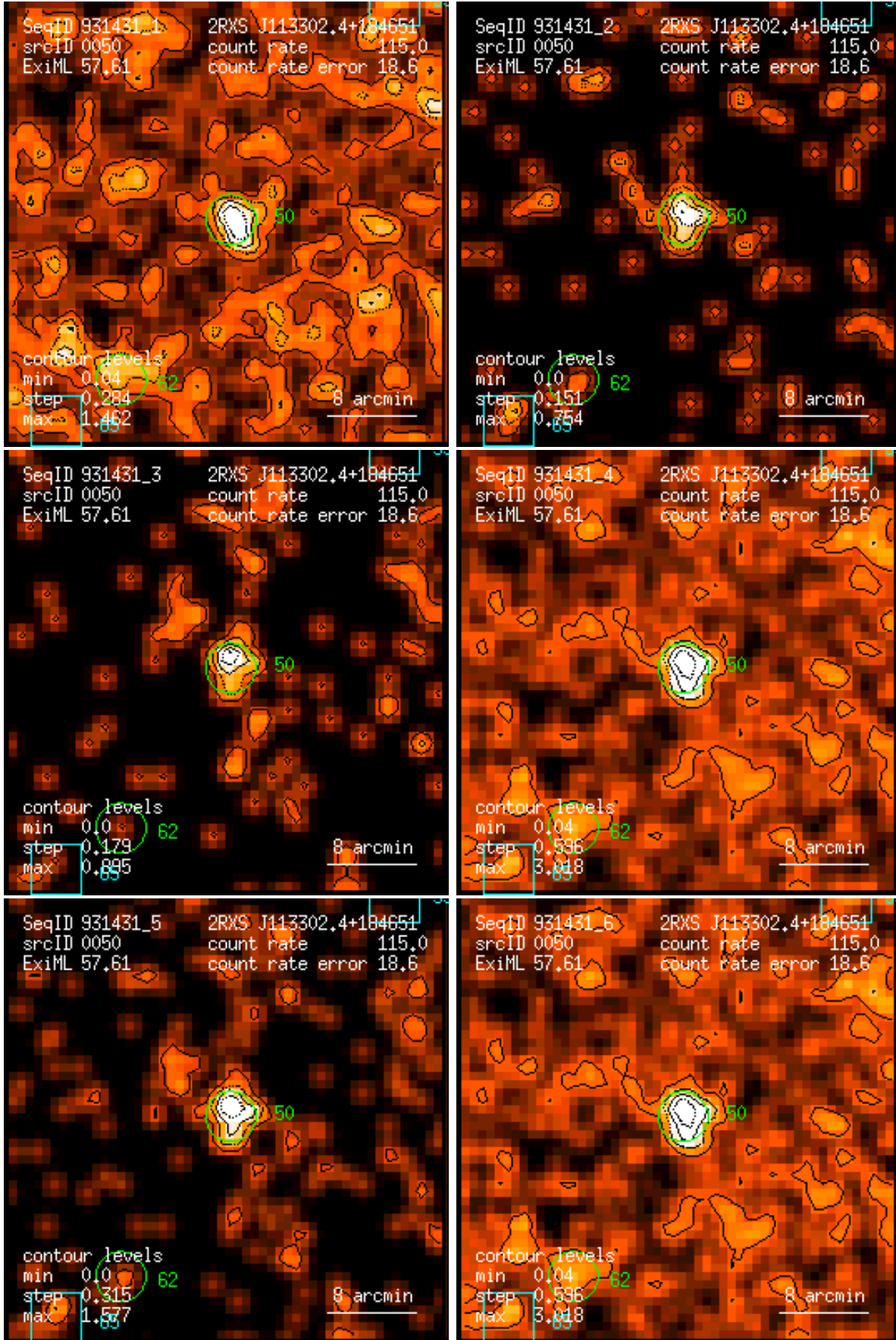
Figure 50: RASS 931431: detection 0050: band rate images, Gaussian filter: (1) PSPC channels 11 – 41, (2) 52 – 90, (3) 91 – 201, (4) 11 – 235, (5) 52 – 201, (6) 11 – 201. Broad band rates in counts/ks. Band rate contour levels in counts/ks/arcmin 2 .
