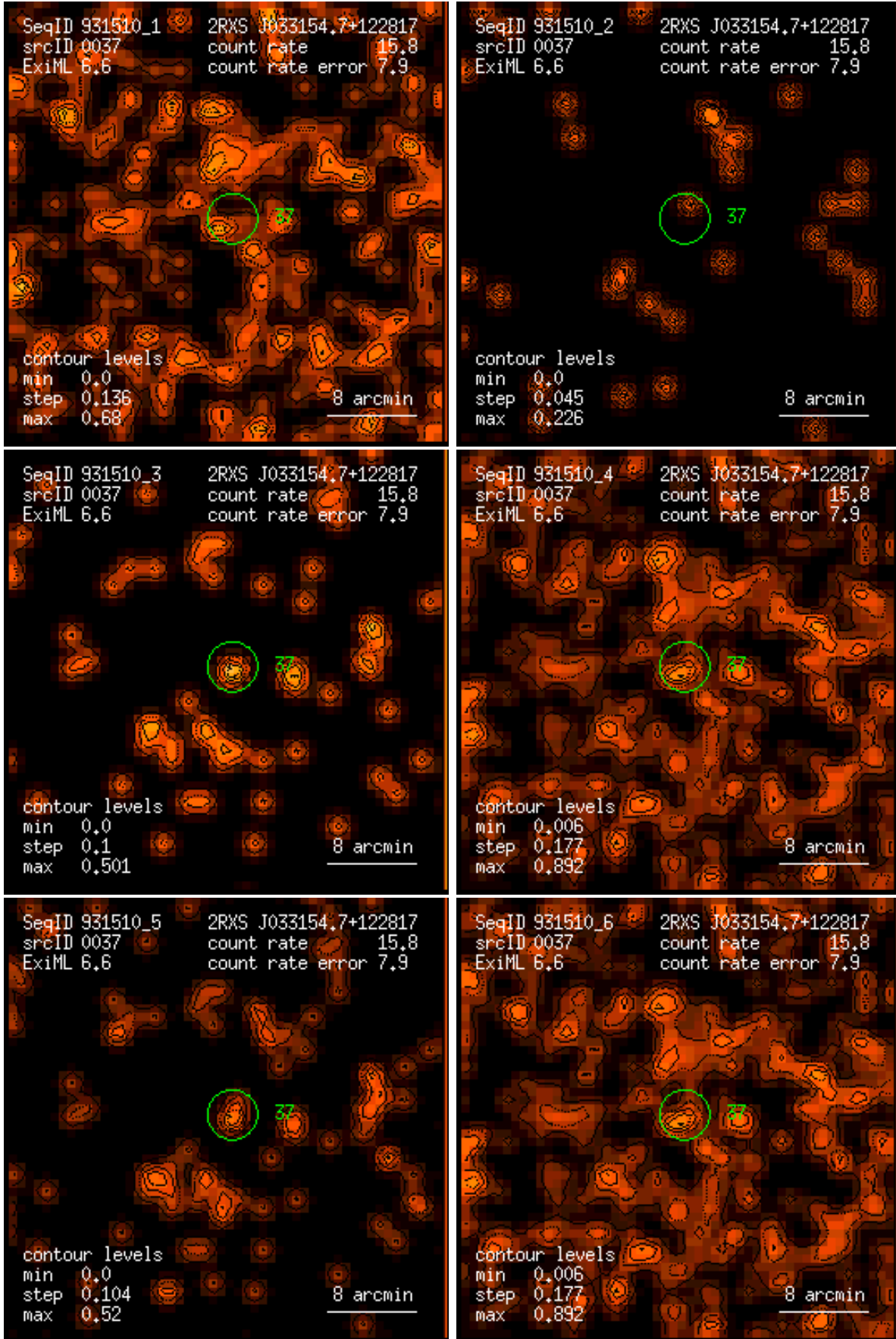
Figure 37: RASS 931510: detection 0037: band rate images, Gaussian filter: (1) PSPC channels 11 – 41, (2) 52 – 90, (3) 91 – 201, (4) 11 – 235, (5) 52 – 201, (6) 11 – 201. Broad band rates in counts/ks. Band rate contour levels in counts/ks/arcmin 2 .
