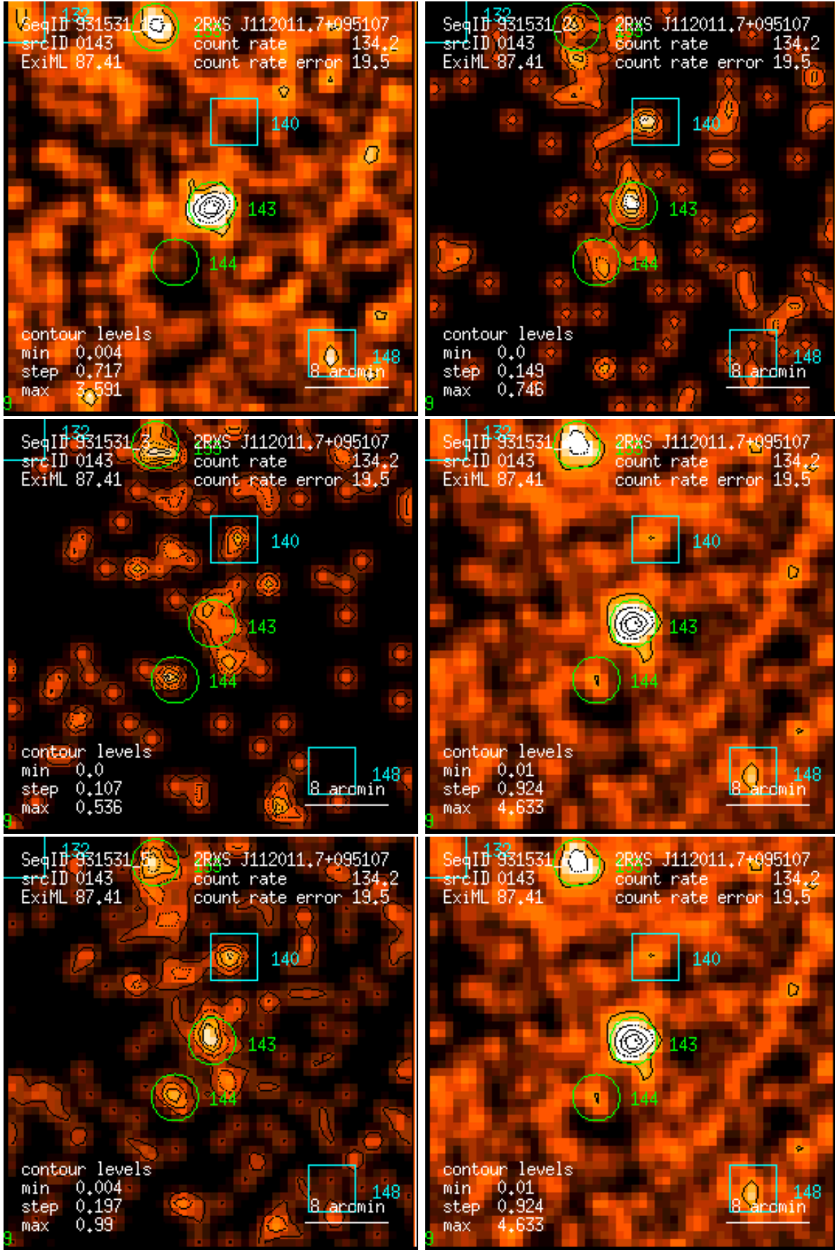
Figure 143: RASS 931531: detection 0143: band rate images, Gaussian filter: (1) PSPC channels 11 – 41, (2) 52 – 90, (3) 91 – 201, (4) 11 – 235, (5) 52 – 201, (6) 11 – 201. Broad band rates in counts/ks. Band rate contour levels in counts/ks/arcmin 2 .
