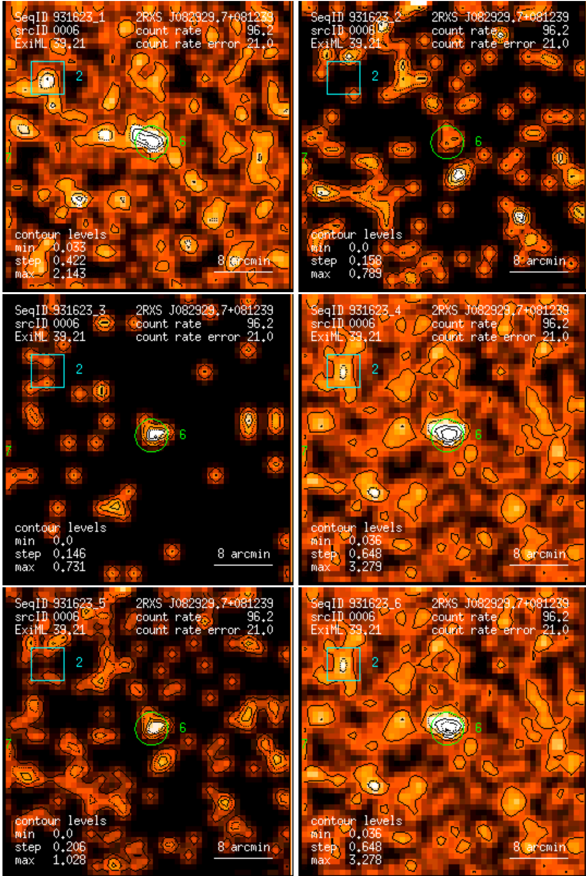
Figure 6: RASS 931623: detection 0006: band rate images, Gaussian filter: (1) PSC channels 11 – 41, (2) 52 – 90, (3) 91 – 201, (4) 11 – 235, (5) 52 – 201, (6) 11 – 201. Broad band rates in counts/ks. Band rate contour levels in counts/ks/arcmin 2 .
