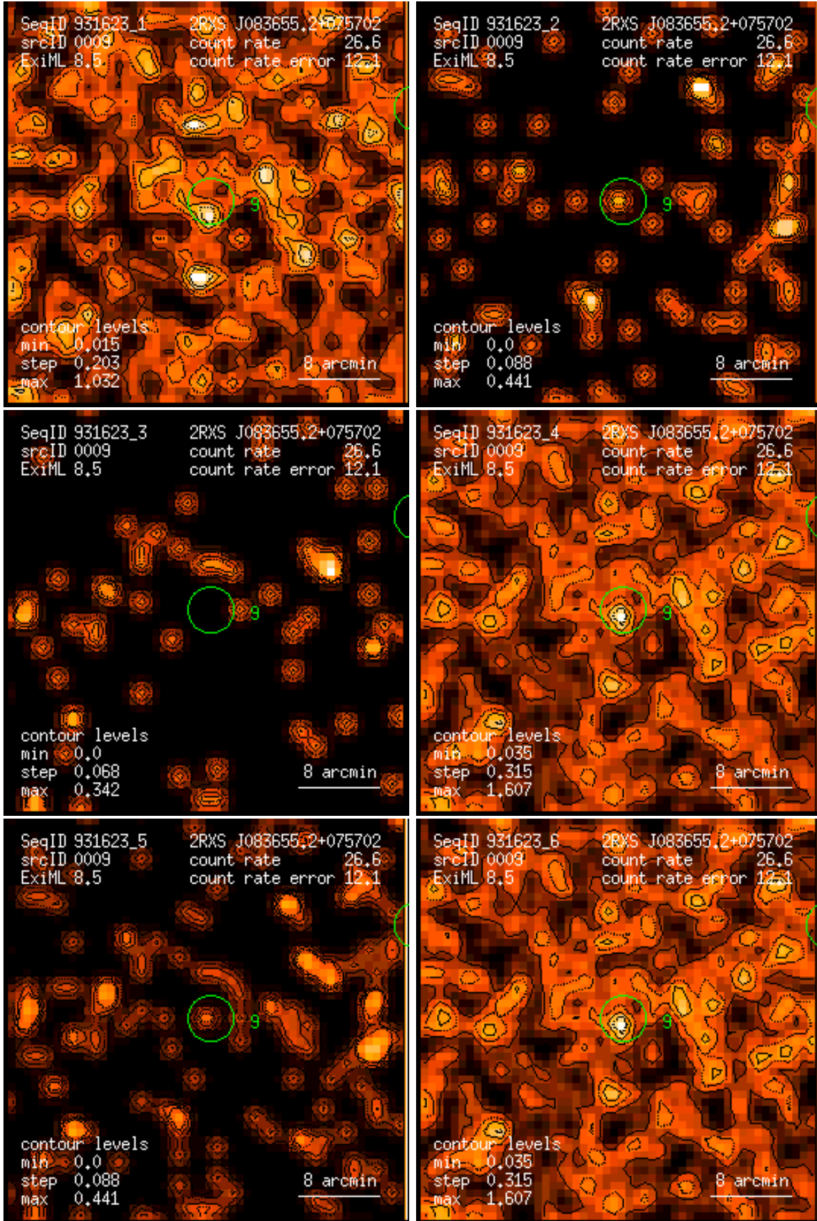
Figure 9: RASS 931623: detection 0009: band rate images, Gaussian filter: (1) PSPC channels 11 – 41, (2) 52 – 90, (3) 91 – 201, (4) 11 – 235, (5) 52 – 201, (6) 11 – 201. Broad band rates in counts/ks. Band rate contour levels in counts/ks/arcmin 2 .
