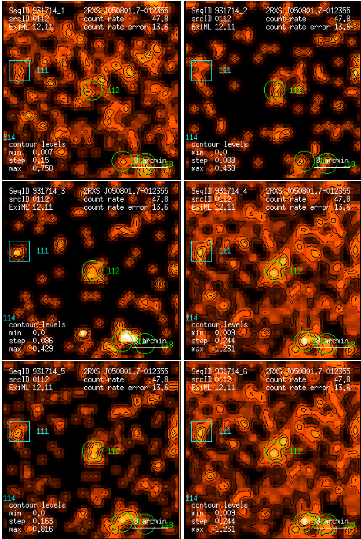
Figure 112: RASS 931714: detection 0112: band rate images, Gaussian filter: (1) PSC channels 11 – 41, (2) 52 – 90, (3) 91 – 201, (4) 11 – 235, (5) 52 – 201, (6) 11 – 201. Broad band rates in counts/ks. Band rate contour levels in counts/ks/arcmin 2 .
