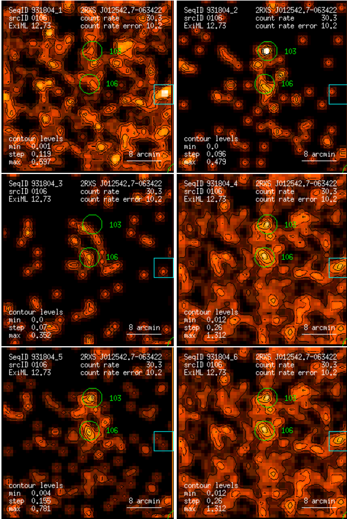
Figure 106: RASS 931804: detection 0106: band rate images, Gaussian filter: (1) PSPC channels 11 – 41, (2) 52 – 90, (3) 91 – 201, (4) 11 – 235, (5) 52 – 201, (6) 11 – 201. Broad band rates in counts/ks. Band rate contour levels in counts/ks/arcmin 2 .
