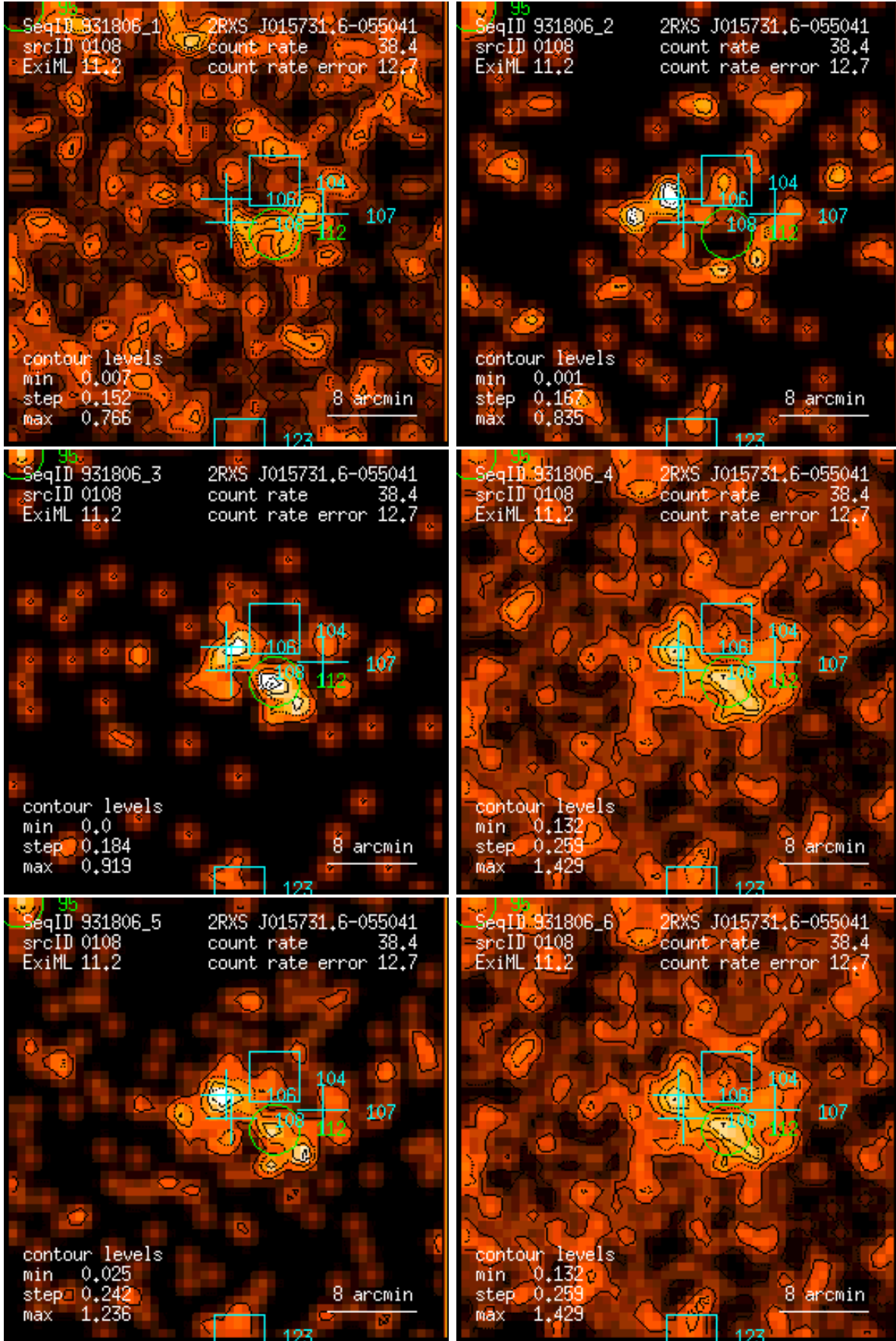
Figure 108: RASS 931806: detection 0108: band rate images, Gaussian filter: (1) PSPC channels 11 – 41, (2) 52 – 90, (3) 91 – 201, (4) 11 – 235, (5) 52 – 201, (6) 11 – 201. Broad band rates in counts/ks. Band rate contour levels in counts/ks/arcmin 2 .
