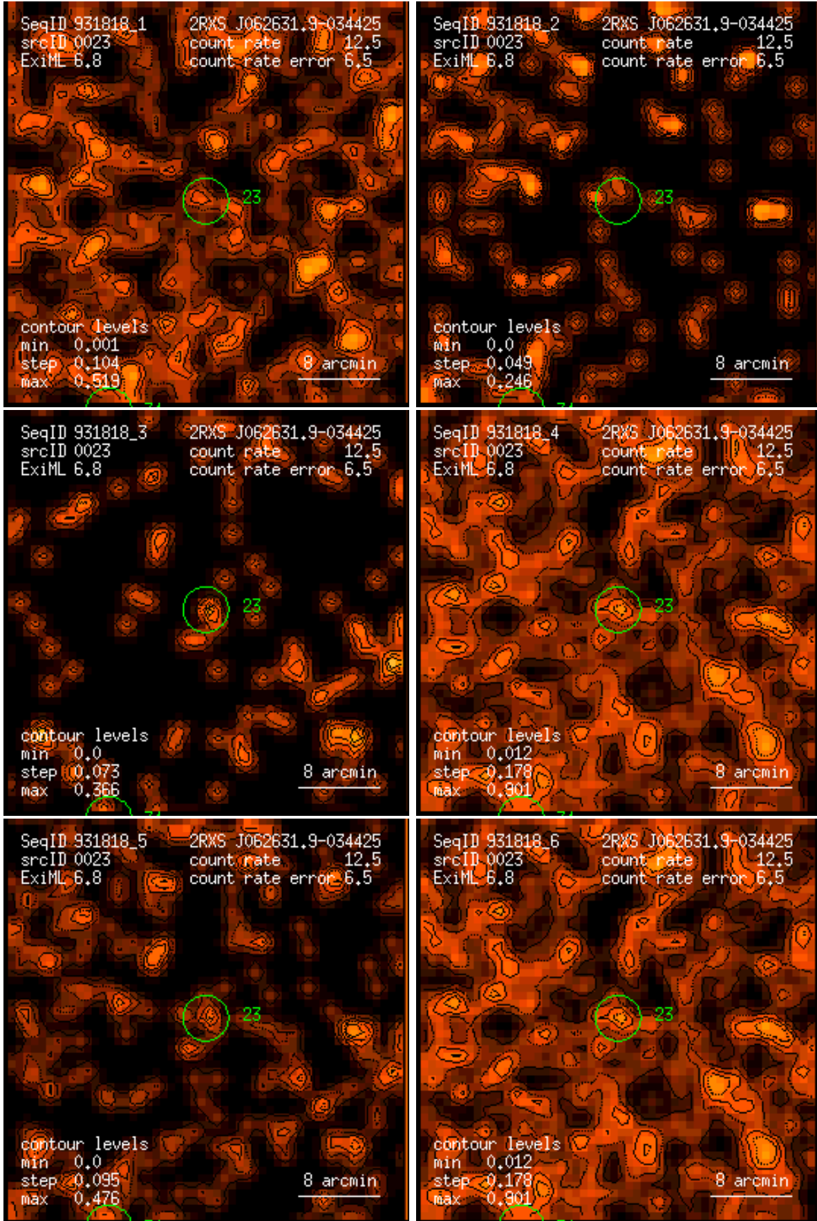
Figure 23: RASS 931818: detection 0023: band rate images, Gaussian filter: (1) PSPC channels 11 – 41, (2) 52 – 90, (3) 91 – 201, (4) 11 – 235, (5) 52 – 201, (6) 11 – 201. Broad band rates in counts/ks. Band rate contour levels in counts/ks/arcmin 2 .
