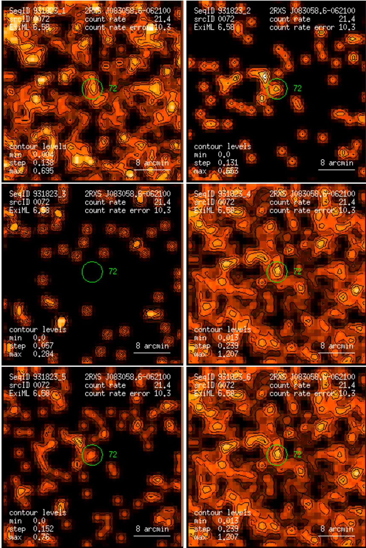
Figure 72: RASS 931823: detection 0072: band rate images, Gaussian filter: (1) PSPC channels 11 – 41, (2) 52 – 90, (3) 91 – 201, (4) 11 – 235, (5) 52 – 201, (6) 11 – 201. Broad band rates in counts/ks. Band rate contour levels in counts/ks/arcmin 2 .
