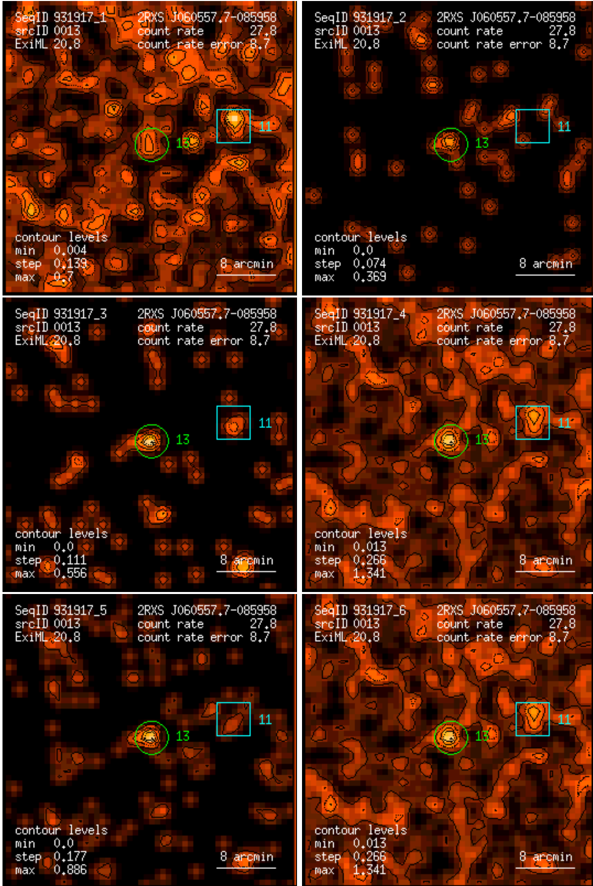
Figure 13: RASS 931917: detection 0013: band rate images, Gaussian filter: (1) PSPC channels 11 – 41, (2) 52 – 90, (3) 91 – 201, (4) 11 – 235, (5) 52 – 201, (6) 11 – 201. Broad band rates in counts/ks. Band rate contour levels in counts/ks/arcmin 2 .
