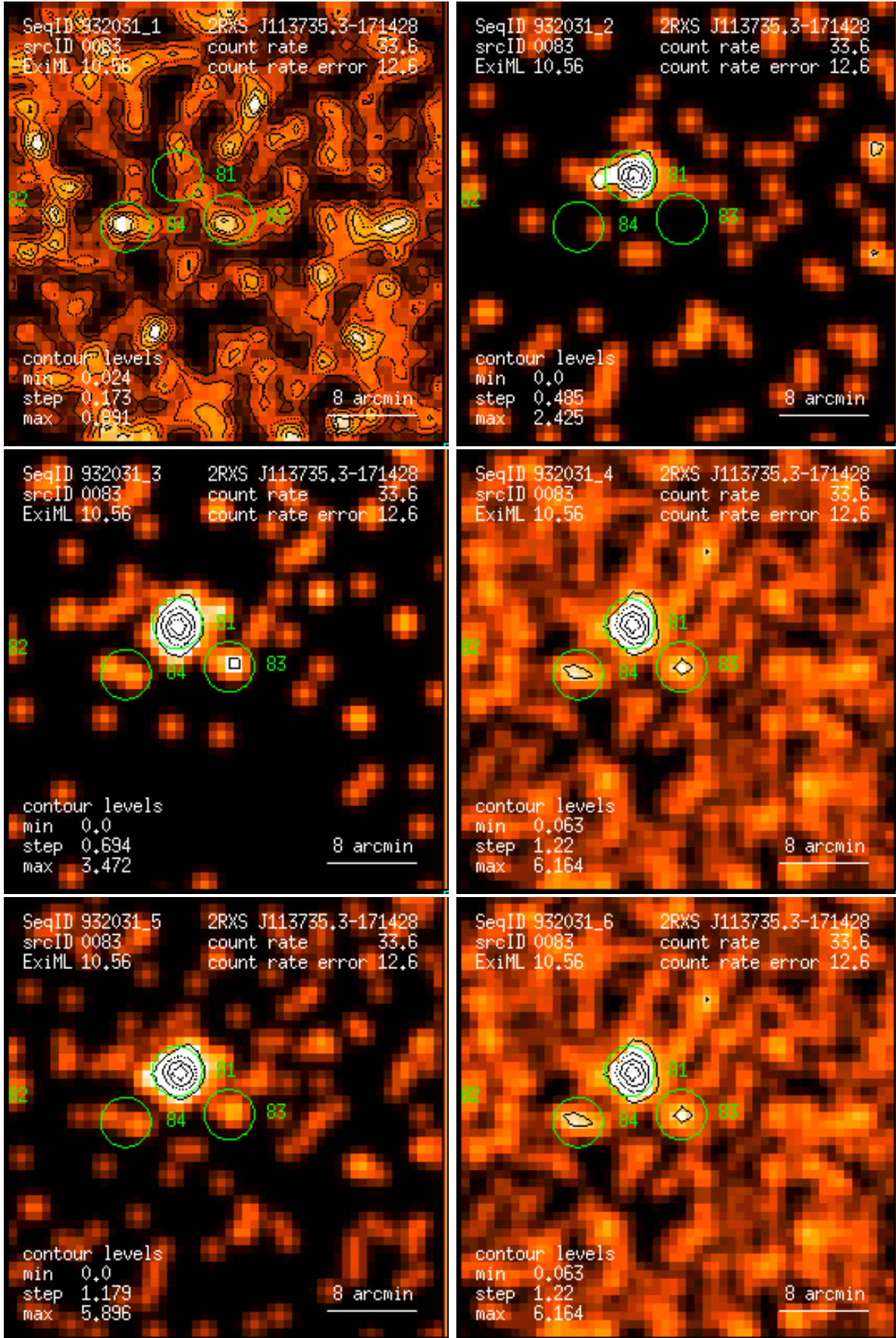
Figure 83: RASS 932031: detection 0083: band rate images, Gaussian filter: (1) PSPC channels 11 – 41, (2) 52 – 90, (3) 91 – 201, (4) 11 – 235, (5) 52 – 201, (6) 11 – 201. Broad band rates in counts/ks. Band rate contour levels in counts/ks/arcmin 2 .
