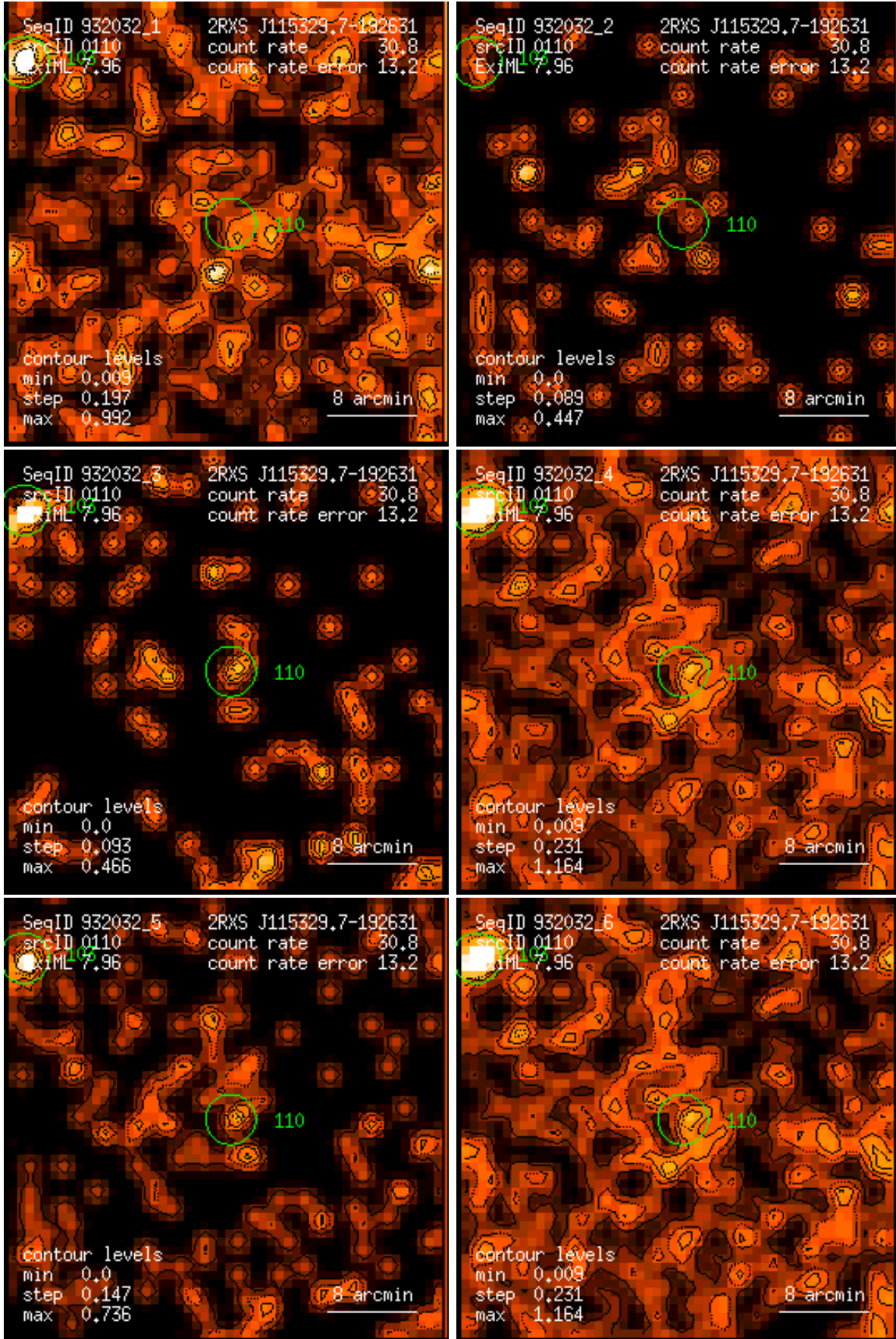
Figure 110: RASS 932032: detection 0110: band rate images, Gaussian filter: (1) PSPC channels 11 – 41, (2) 52 – 90, (3) 91 – 201, (4) 11 – 235, (5) 52 – 201, (6) 11 – 201. Broad band rates in counts/ks. Band rate contour levels in counts/ks/arcmin 2 .
