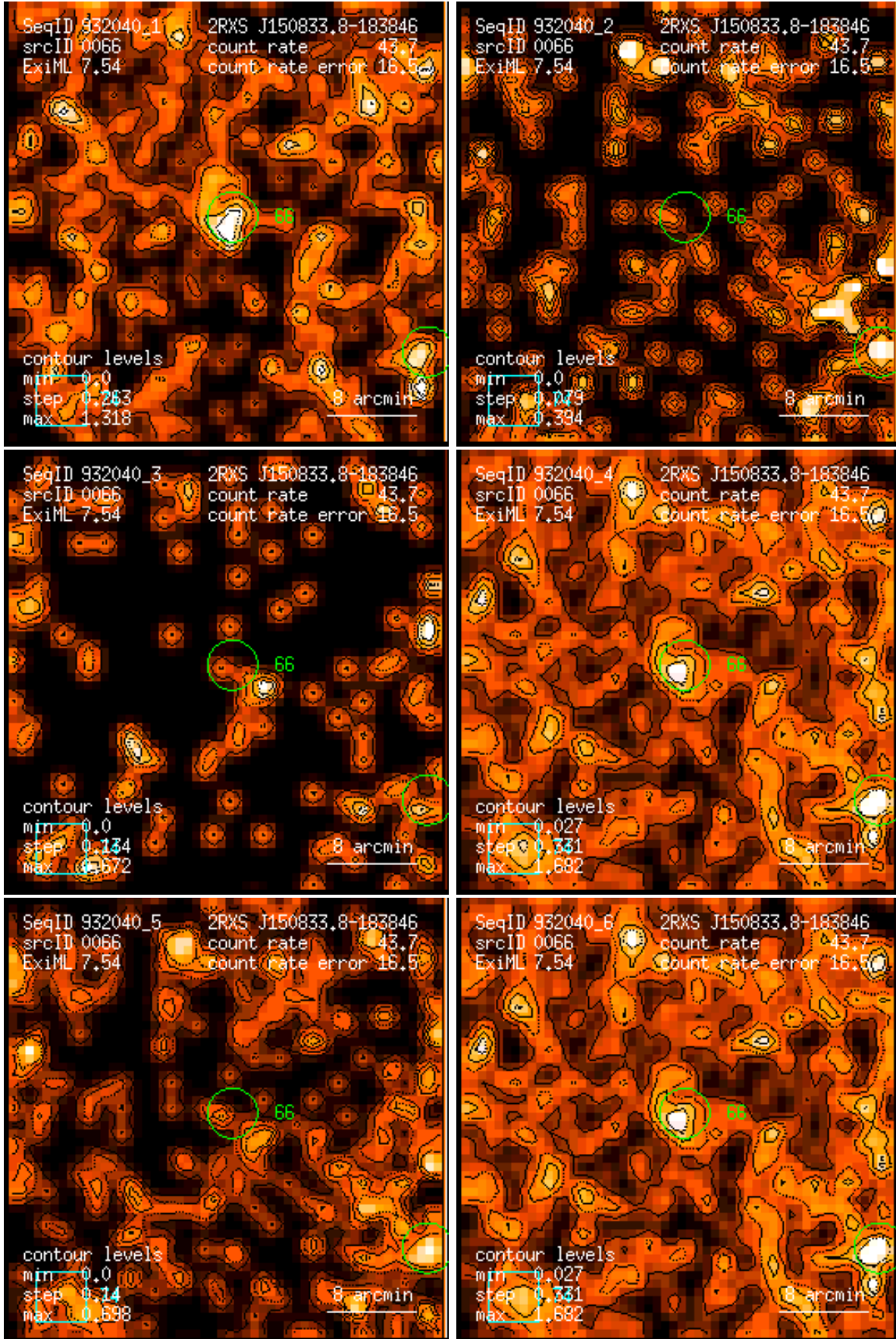
Figure 66: RASS 932040: detection 0066: band rate images, Gaussian filter: (1) PSPC channels 11 – 41, (2) 52 – 90, (3) 91 – 201, (4) 11 – 235, (5) 52 – 201, (6) 11 – 201. Broad band rates in counts/ks. Band rate contour levels in counts/ks/arcmin 2 .
