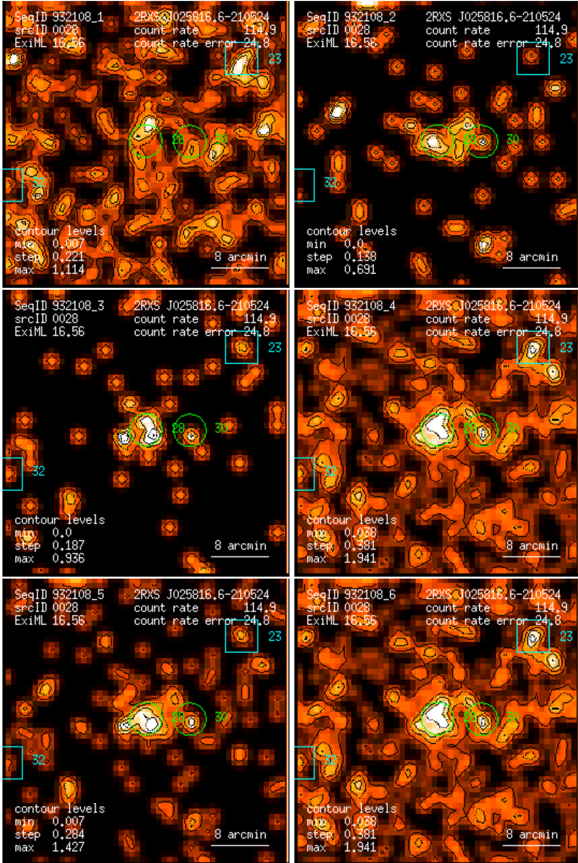
Figure 28: RASS 932108: detection 0028: band rate images, Gaussian filter: (1) PSPC channels 11 – 41, (2) 52 – 90, (3) 91 – 201, (4) 11 – 235, (5) 52 – 201, (6) 11 – 201. Broad band rates in counts/ks. Band rate contour levels in counts/ks/arcmin 2 .
