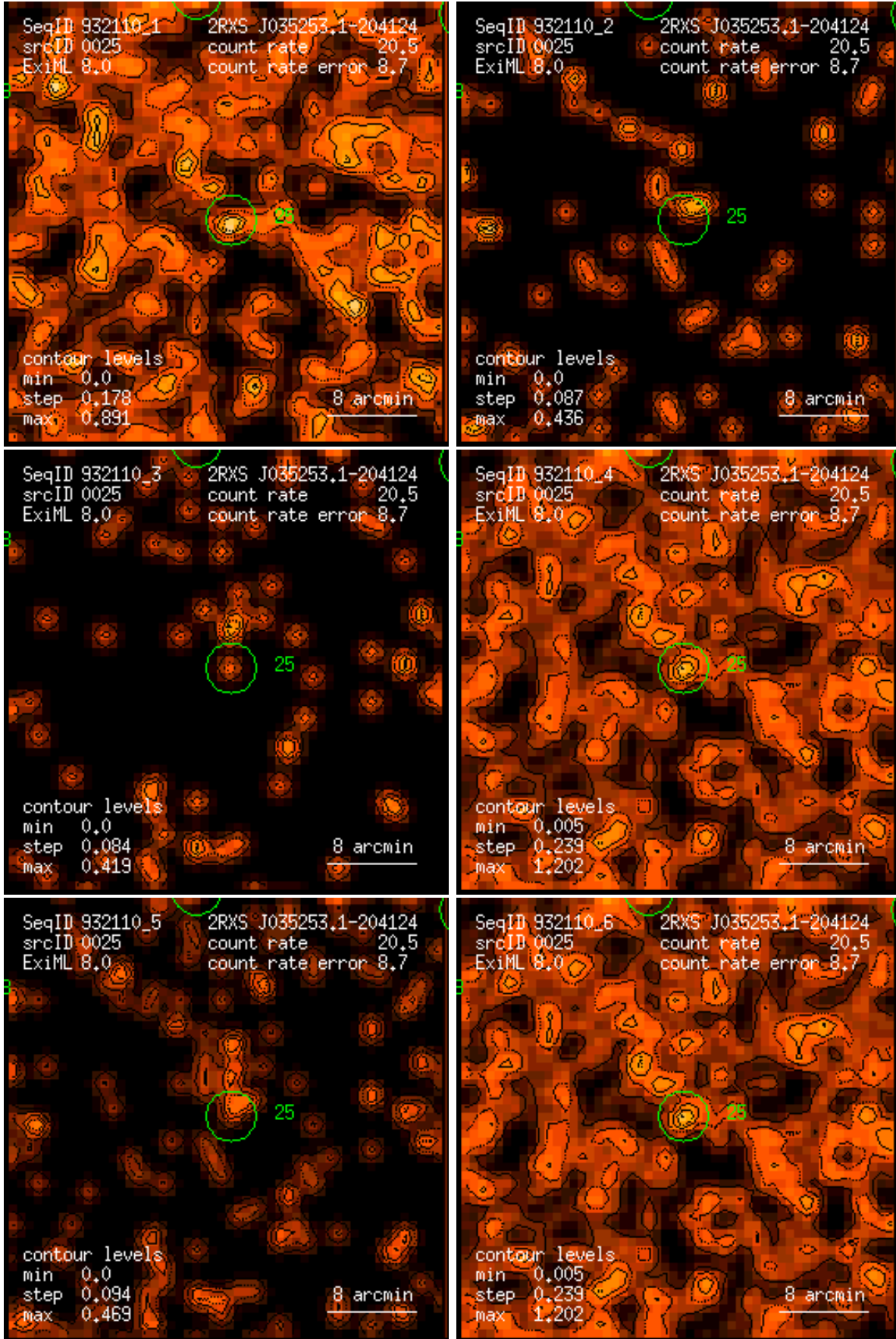
Figure 25: RASS 932110: detection 0025: band rate images, Gaussian filter: (1) PSPC channels 11 – 41, (2) 52 – 90, (3) 91 – 201, (4) 11 – 235, (5) 52 – 201, (6) 11 – 201. Broad band rates in counts/ks. Band rate contour levels in counts/ks/arcmin 2 .
