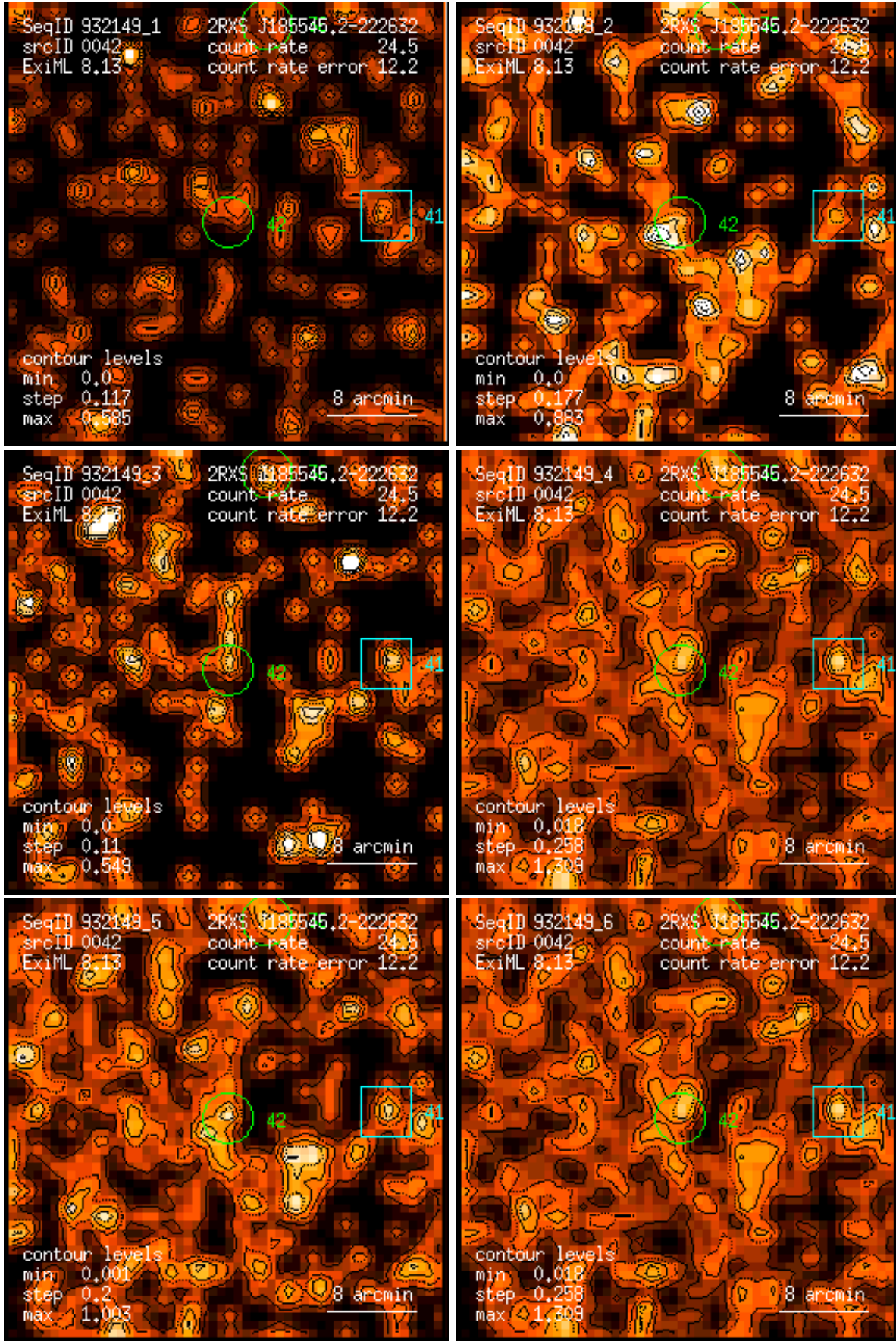
Figure 42: RASS 932149: detection 0042: band rate images, Gaussian filter: (1) PSPC channels 11 – 41, (2) 52 – 90, (3) 91 – 201, (4) 11 – 235, (5) 52 – 201, (6) 11 – 201. Broad band rates in counts/ks. Band rate contour levels in counts/ks/arcmin 2 .
