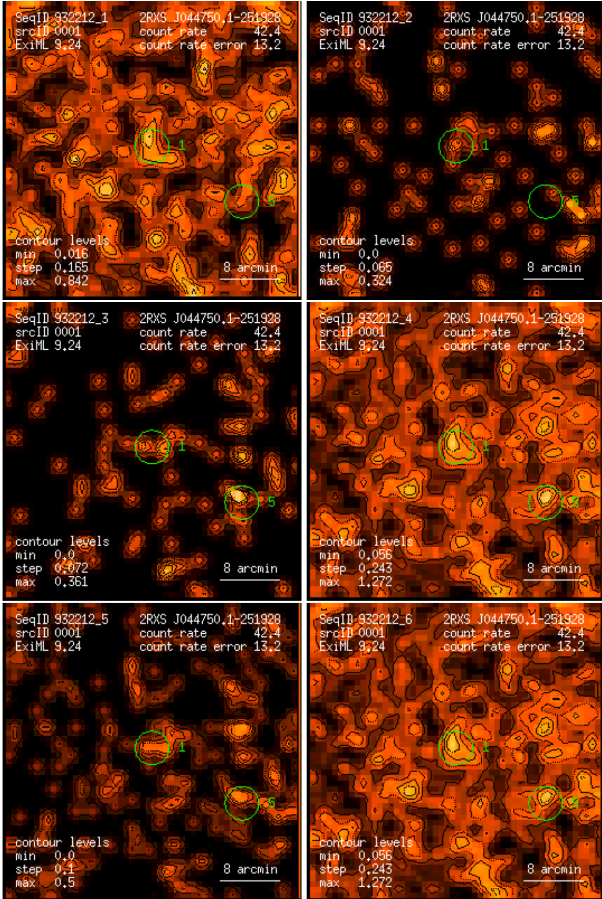
Figure 1: RASS 932212: detection 0001: band rate images, Gaussian filter: (1) PSPC channels 11 – 41, (2) 52 – 90, (3) 91 – 201, (4) 11 – 235, (5) 52 – 201, (6) 11 – 201. Broad band rates in counts/ks. Band rate contour levels in counts/ks/arcmin 2 .
