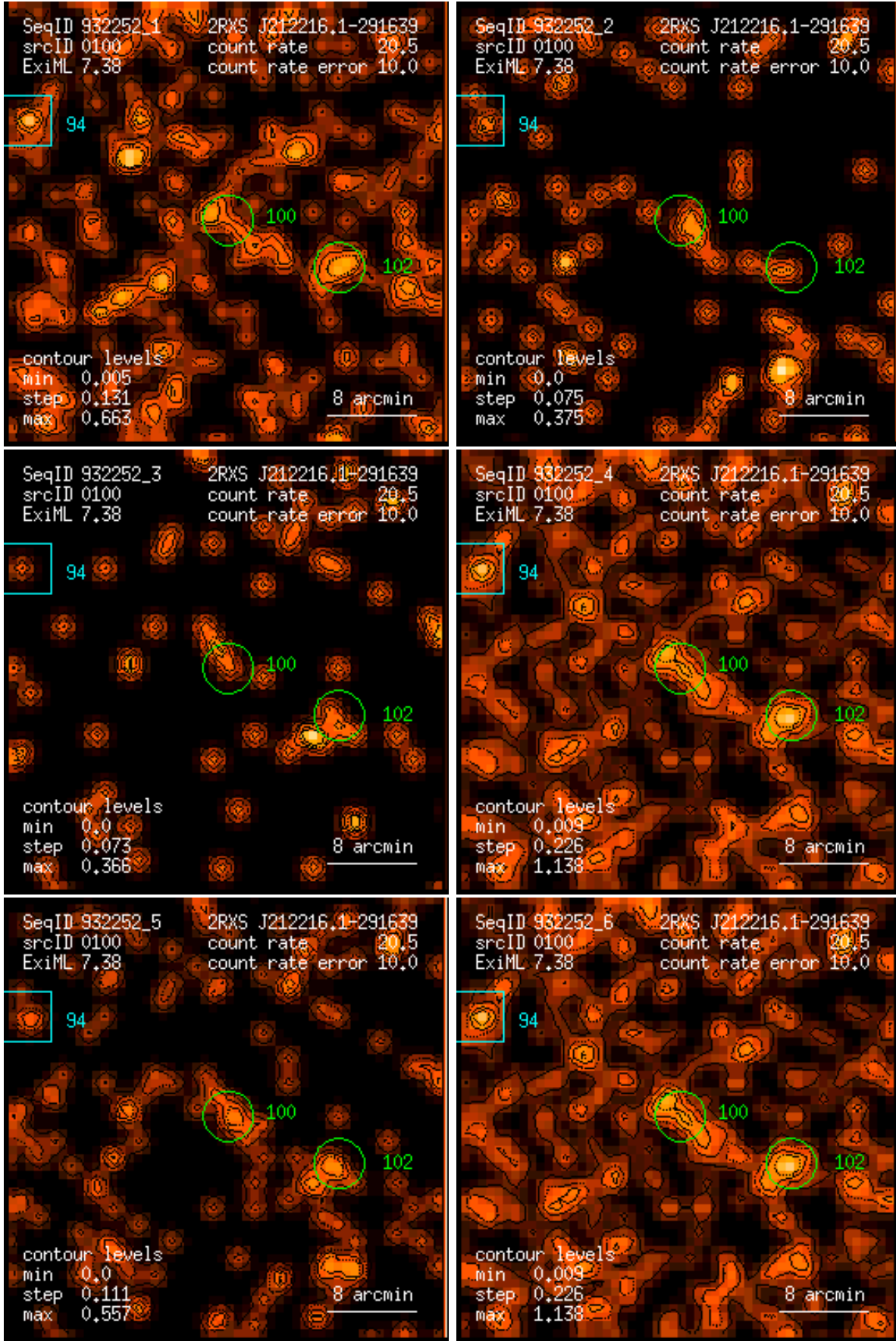
Figure 100: RASS 932252: detection 0100: band rate images, Gaussian filter: (1) PSPC channels 11 – 41, (2) 52 – 90, (3) 91 – 201, (4) 11 – 235, (5) 52 – 201, (6) 11 – 201. Broad band rates in counts/ks. Band rate contour levels in counts/ks/arcmin 2 .
