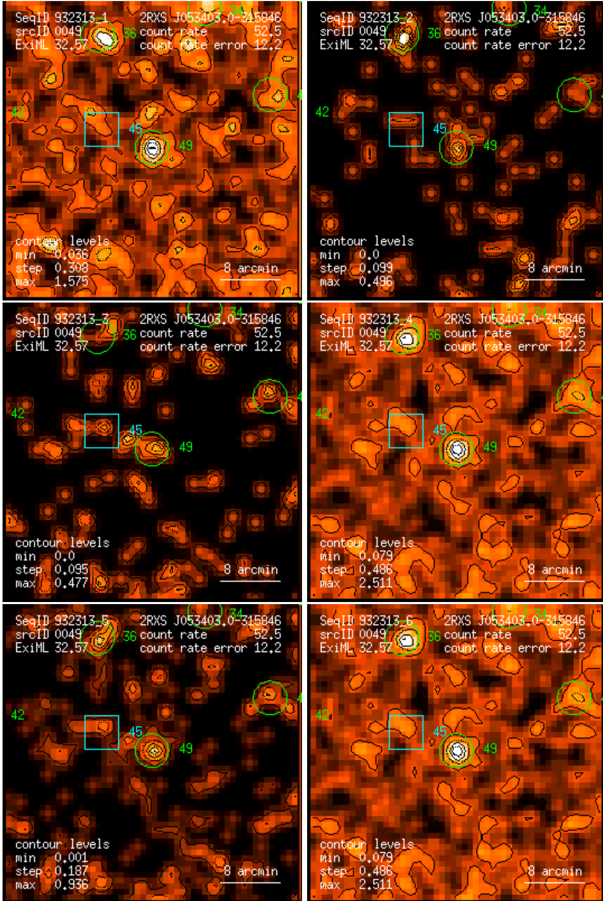
Figure 49: RASS 932313: detection 0049: band rate images, Gaussian filter: (1) PSPC channels 11 – 41, (2) 52 – 90, (3) 91 – 201, (4) 11 – 235, (5) 52 – 201, (6) 11 – 201. Broad band rates in counts/ks. Band rate contour levels in counts/ks/arcmin 2 .
