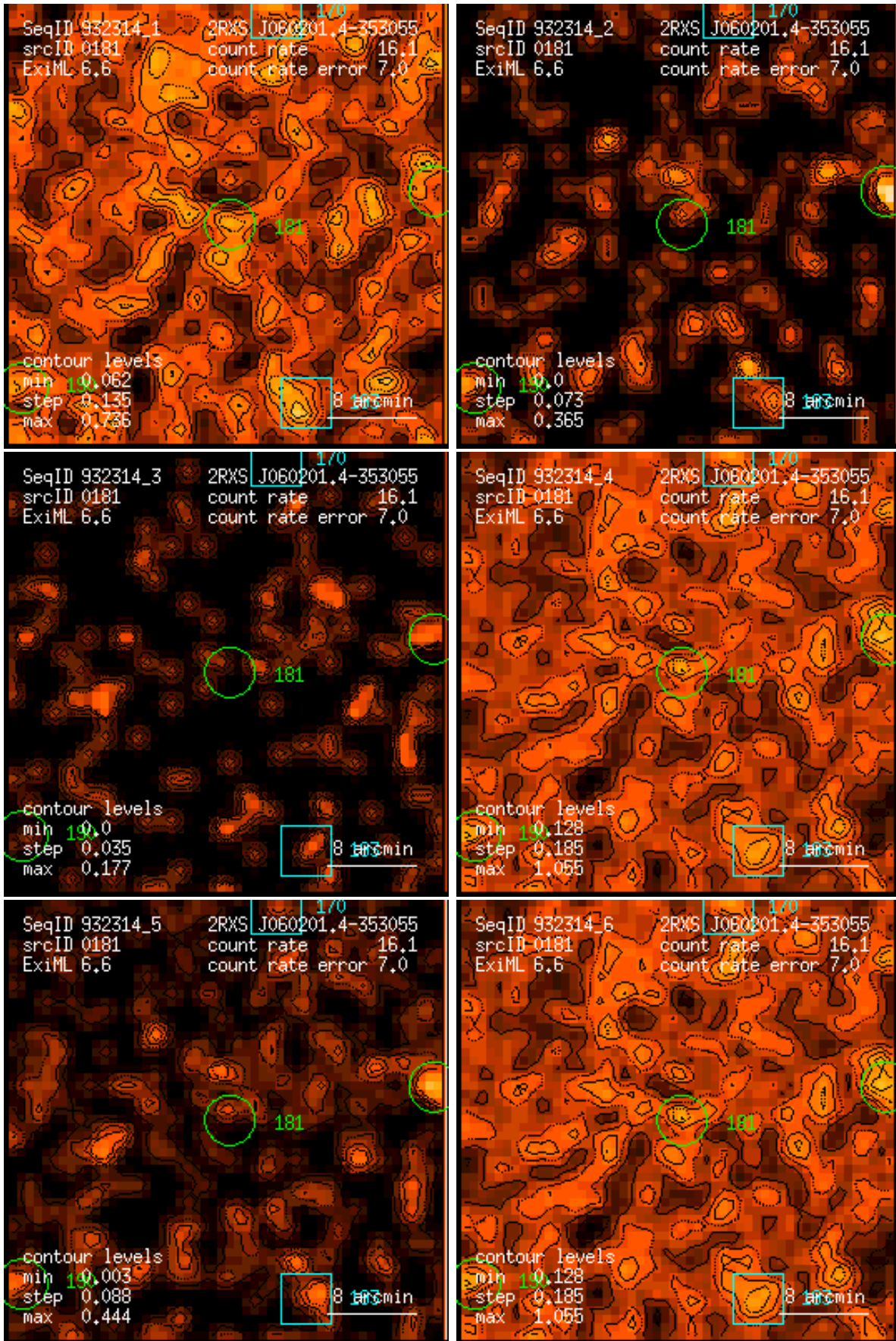
Figure 181: RASS 932314: detection 0181: band rate images, Gaussian filter: (1) PSPC channels 11 – 41, (2) 52 – 90, (3) 91 – 201, (4) 11 – 235, (5) 52 – 201, (6) 11 – 201. Broad band rates in counts/ks. Band rate contour levels in counts/ks/arcmin 2 .
