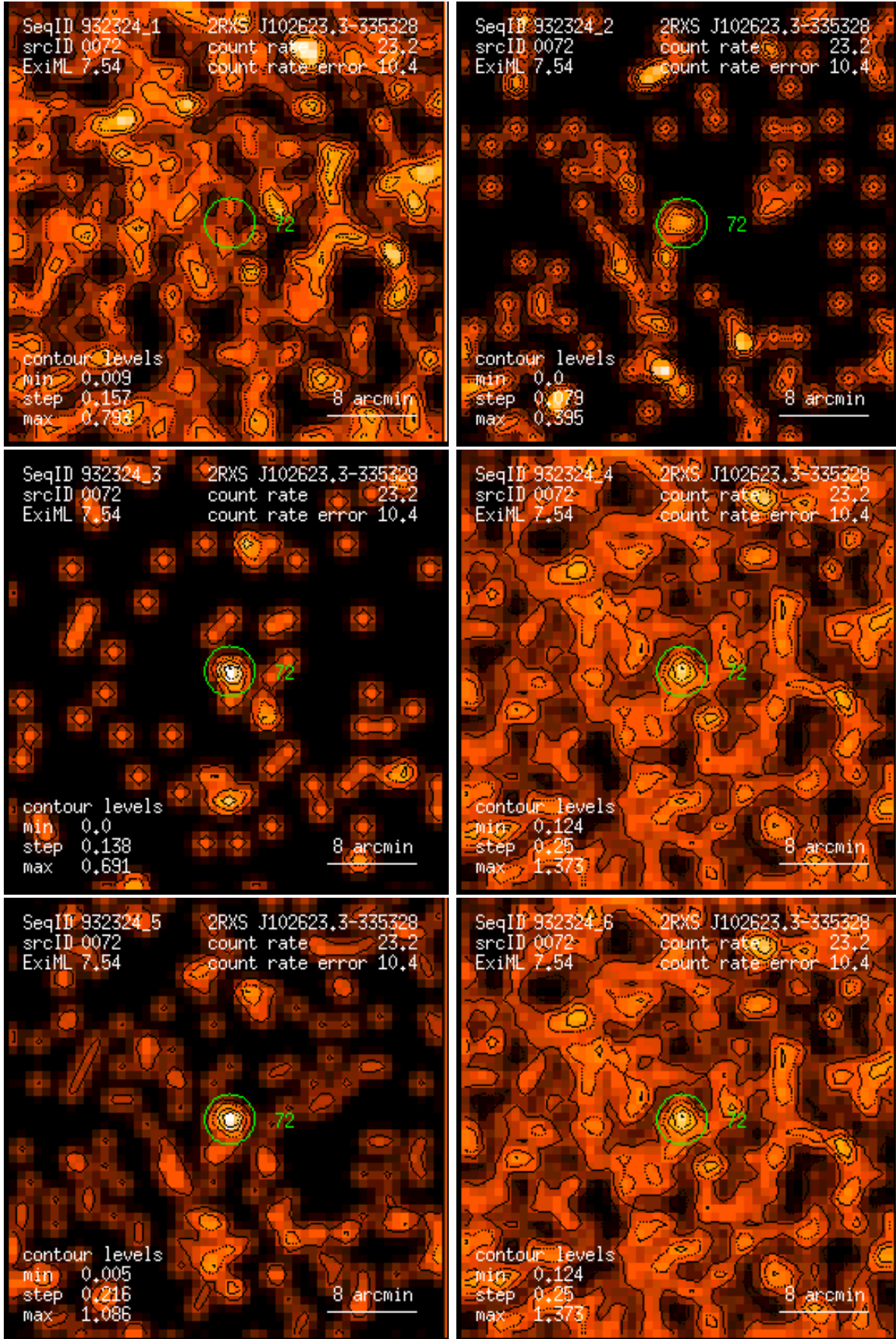
Figure 72: RASS 932324: detection 0072: band rate images, Gaussian filter: (1) PSPC channels 11 – 41, (2) 52 – 90, (3) 91 – 201, (4) 11 – 235, (5) 52 – 201, (6) 11 – 201. Broad band rates in counts/ks. Band rate contour levels in counts/ks/arcmin 2 .
