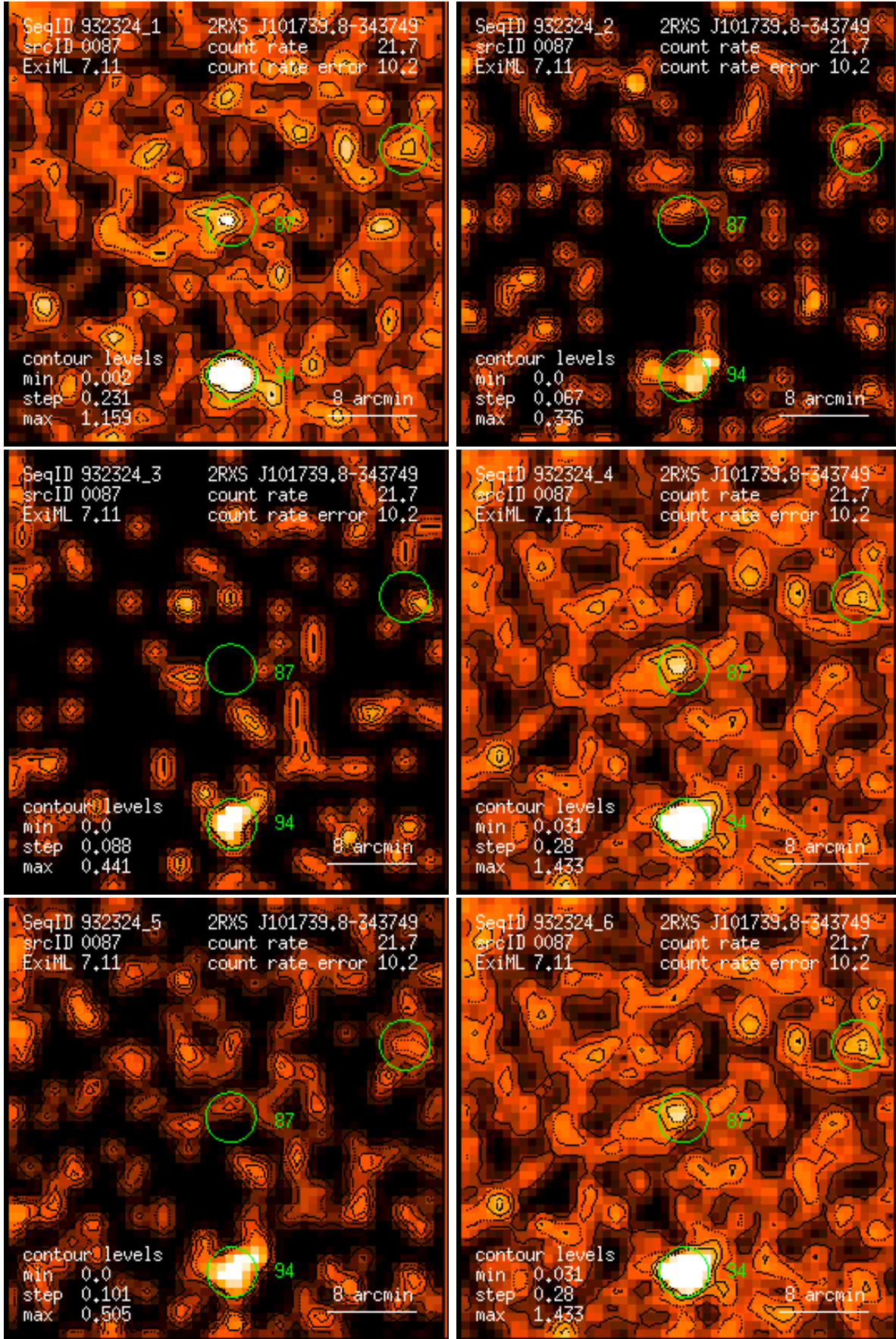
Figure 87: RASS 932324: detection 0087: band rate images, Gaussian filter: (1) PSPC channels 11 – 41, (2) 52 – 90, (3) 91 – 201, (4) 11 – 235, (5) 52 – 201, (6) 11 – 201. Broad band rates in counts/ks. Band rate contour levels in counts/ks/arcmin 2 .
