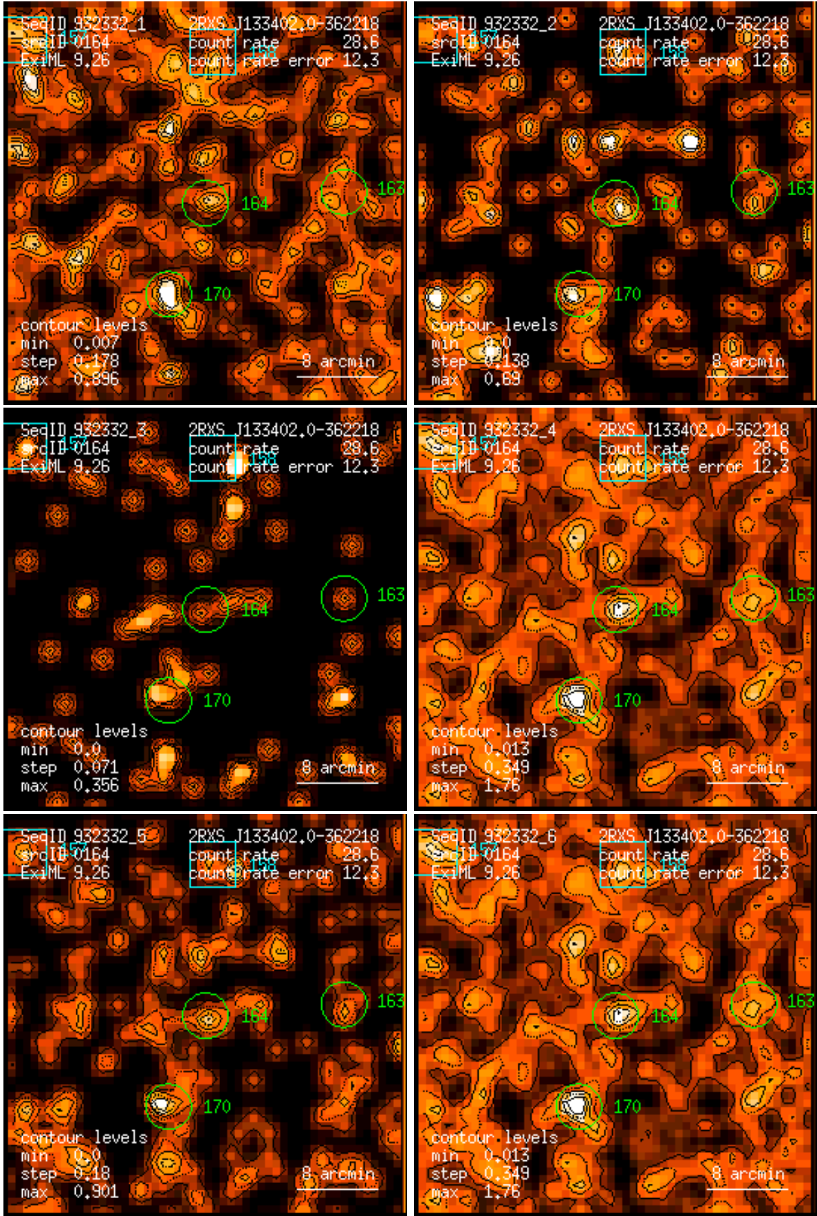
Figure 164: RASS 932332: detection 0164: band rate images, Gaussian filter: (1) PSPC channels 11 – 41, (2) 52 – 90, (3) 91 – 201, (4) 11 – 235, (5) 52 – 201, (6) 11 – 201. Broad band rates in counts/ks. Band rate contour levels in counts/ks/arcmin 2 .
