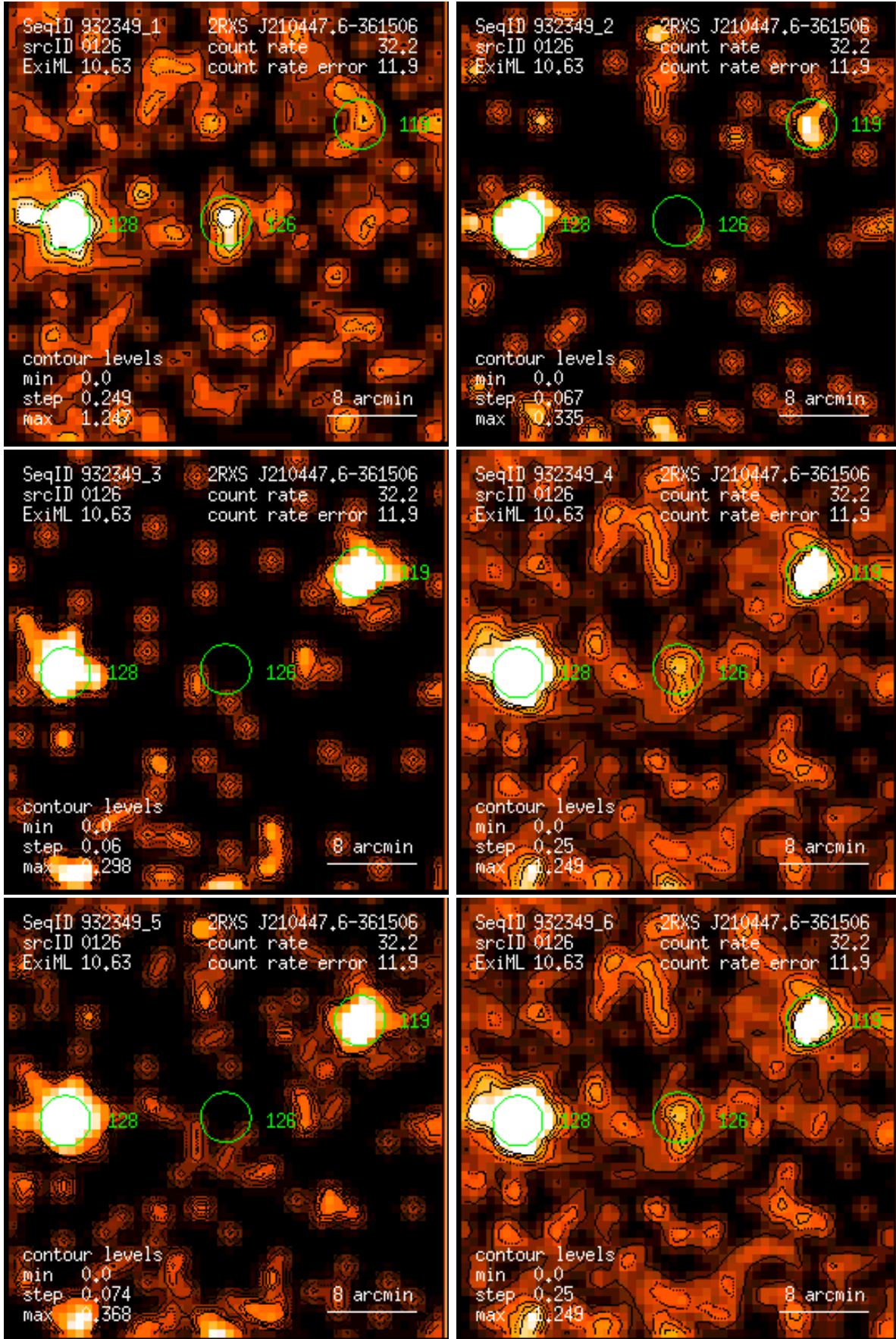
Figure 126: RASS 932349: detection 0126: band rate images, Gaussian filter: (1) PSPC channels 11 – 41, (2) 52 – 90, (3) 91 – 201, (4) 11 – 235, (5) 52 – 201, (6) 11 – 201. Broad band rates in counts/ks. Band rate contour levels in counts/ks/arcmin 2 .
