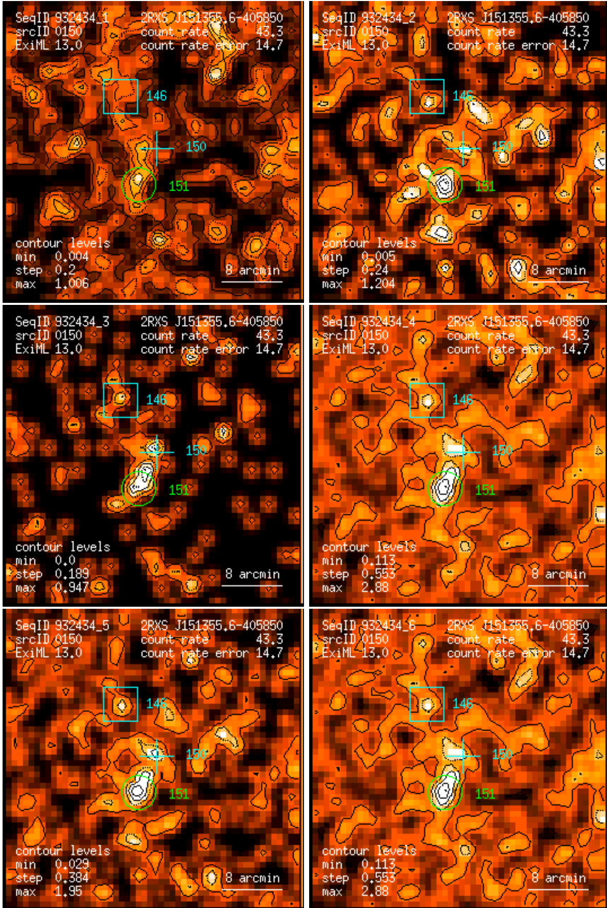
Figure 150: RASS 932434: detection 0150: band rate images, Gaussian filter: (1) PSPC channels 11 – 41, (2) 52 – 90, (3) 91 – 201, (4) 11 – 235, (5) 52 – 201, (6) 11 – 201. Broad band rates in counts/ks. Band rate contour levels in counts/ks/arcmin 2 .
