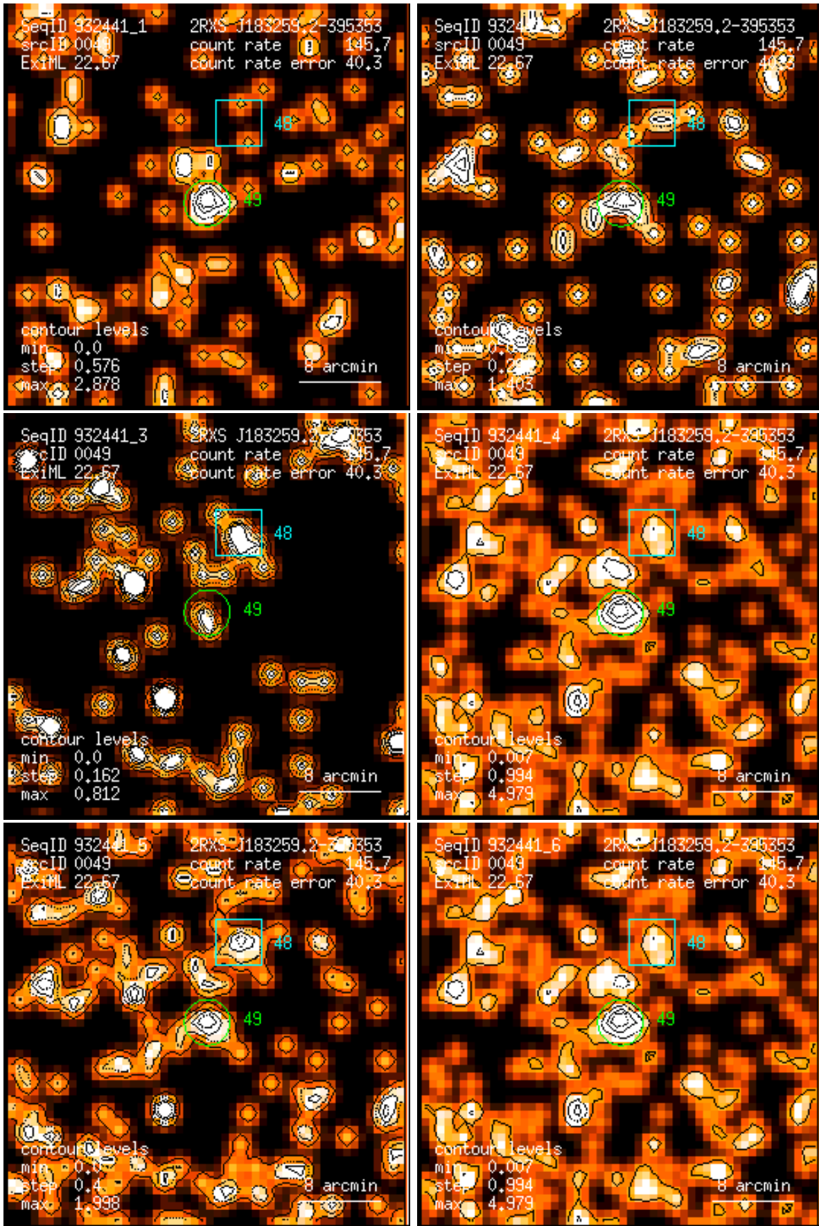
Figure 49: RASS 932441: detection 0049: band rate images, Gaussian filter: (1) PSPC channels 11 – 41, (2) 52 – 90, (3) 91 – 201, (4) 11 – 235, (5) 52 – 201, (6) 11 – 201. Broad band rates in counts/ks. Band rate contour levels in counts/ks/arcmin 2 .
