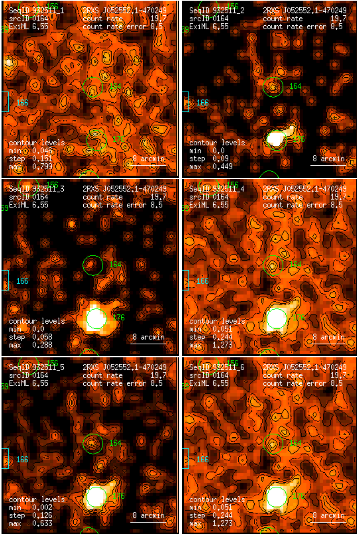
Figure 164: RASS 932511: detection 0164: band rate images, Gaussian filter: (1) PSPC channels 11 – 41, (2) 52 – 90, (3) 91 – 201, (4) 11 – 235, (5) 52 – 201, (6) 11 – 201. Broad band rates in counts/ks. Band rate contour levels in counts/ks/arcmin 2 .
