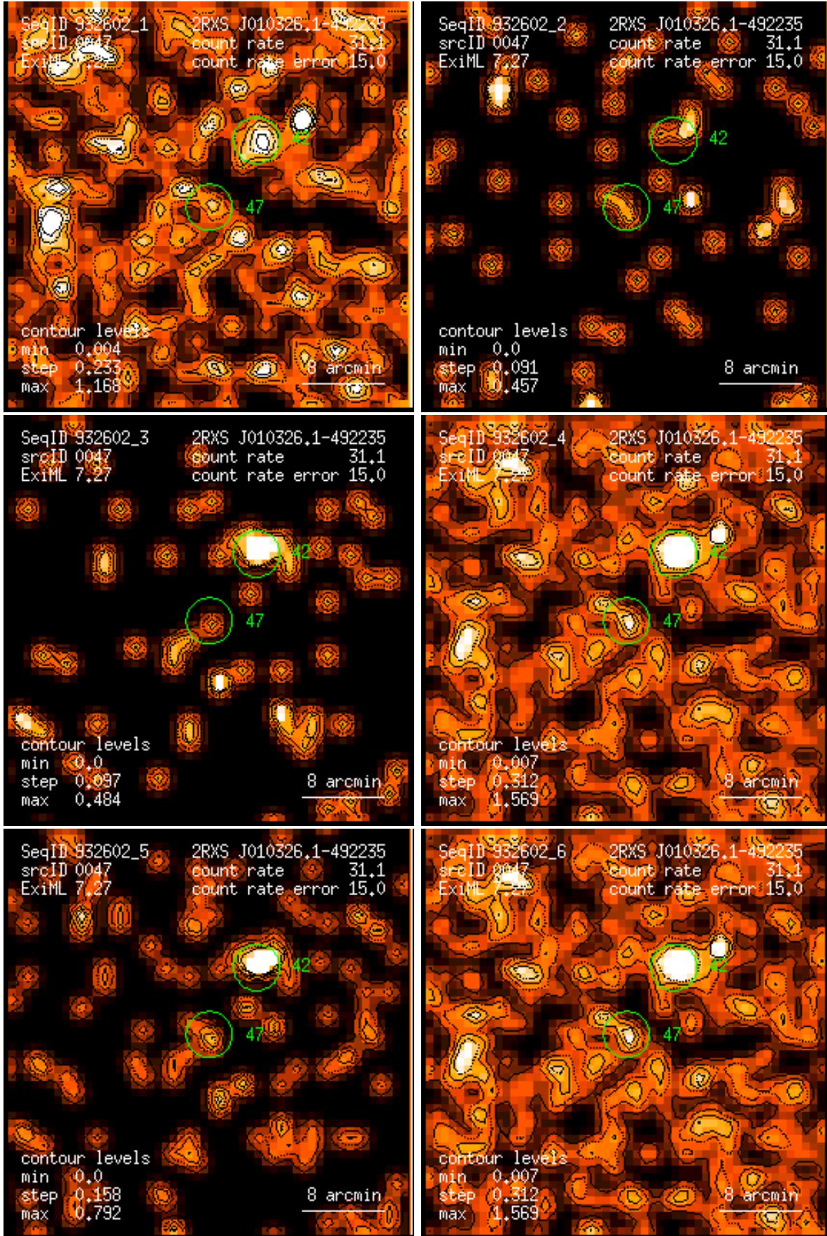
Figure 47: RASS 932602: detection 0047: band rate images, Gaussian filter: (1) PSPC channels 11 – 41, (2) 52 – 90, (3) 91 – 201, (4) 11 – 235, (5) 52 – 201, (6) 11 – 201. Broad band rates in counts/ks. Band rate contour levels in counts/ks/arcmin 2 .
