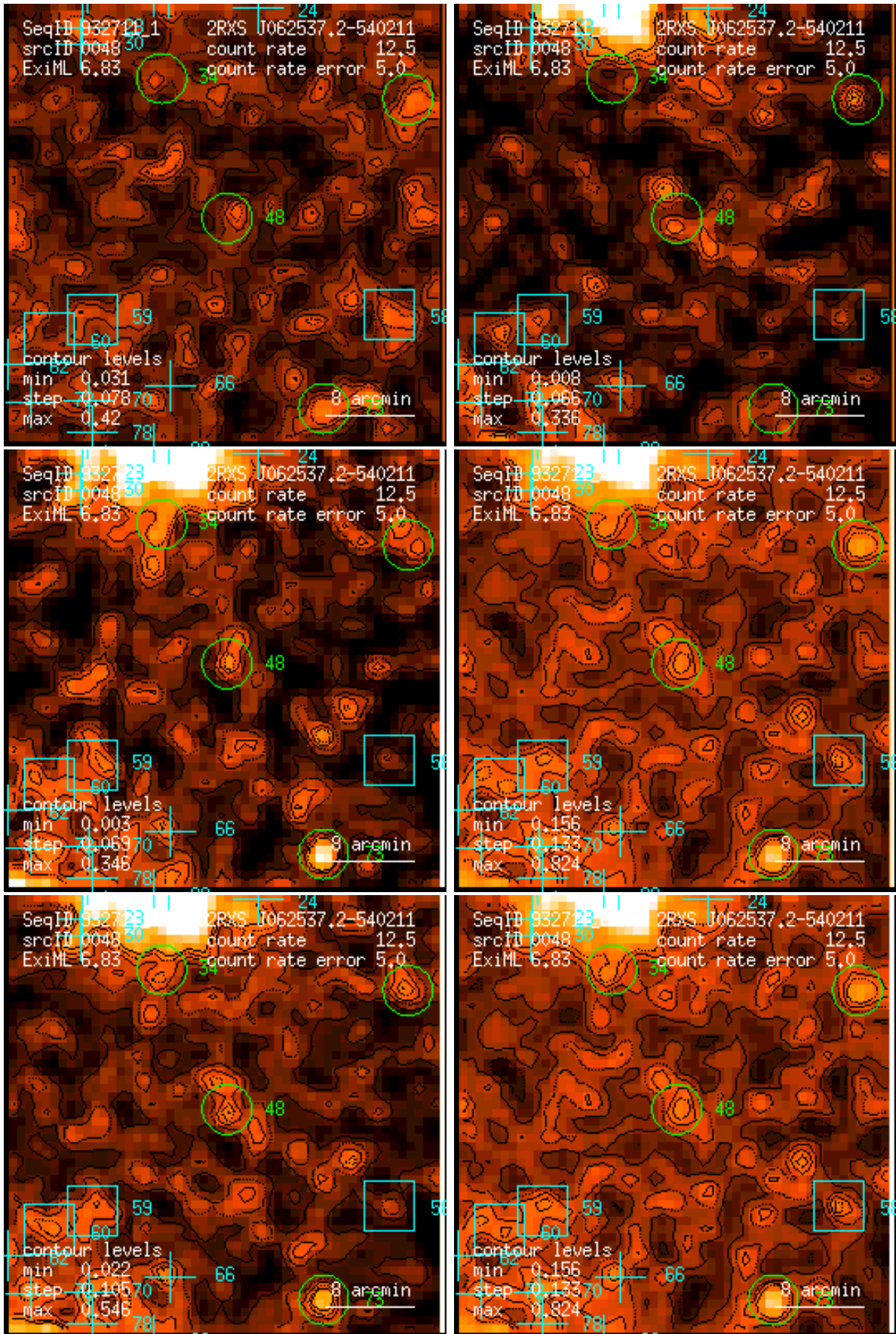
Figure 48: RASS 932711: detection 0048: band rate images, Gaussian filter: (1) PSPC channels 11 – 41, (2) 52 – 90, (3) 91 – 201, (4) 11 – 235, (5) 52 – 201, (6) 11 – 201. Broad band rates in counts/ks. Band rate contour levels in counts/ks/arcmin 2 .
