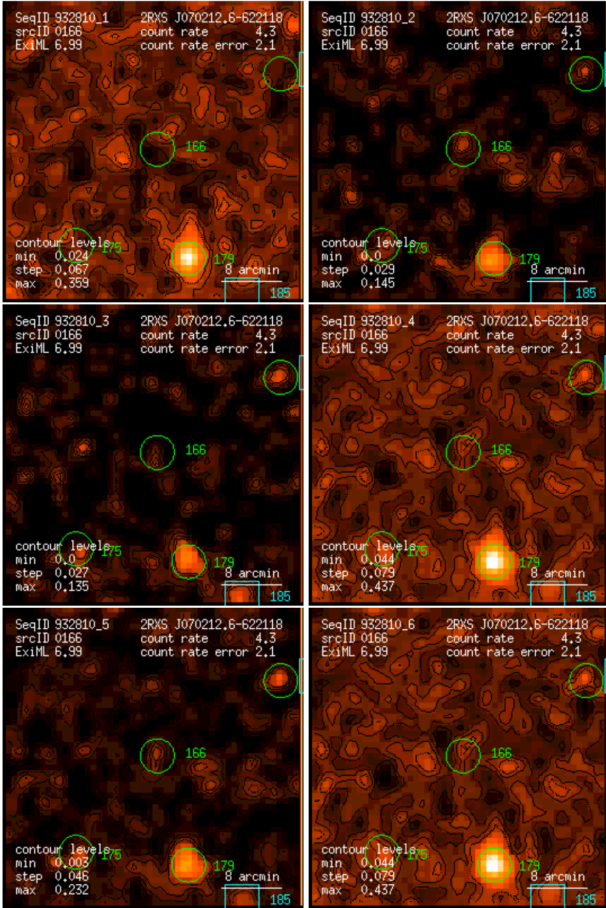
Figure 166: RASS 932810: detection 0166: band rate images, Gaussian filter: (1) PSPC channels 11 – 41, (2) 52 – 90, (3) 91 – 201, (4) 11 – 235, (5) 52 – 201, (6) 11 – 201. Broad band rates in counts/ks. Band rate contour levels in counts/ks/arcmin 2 .
