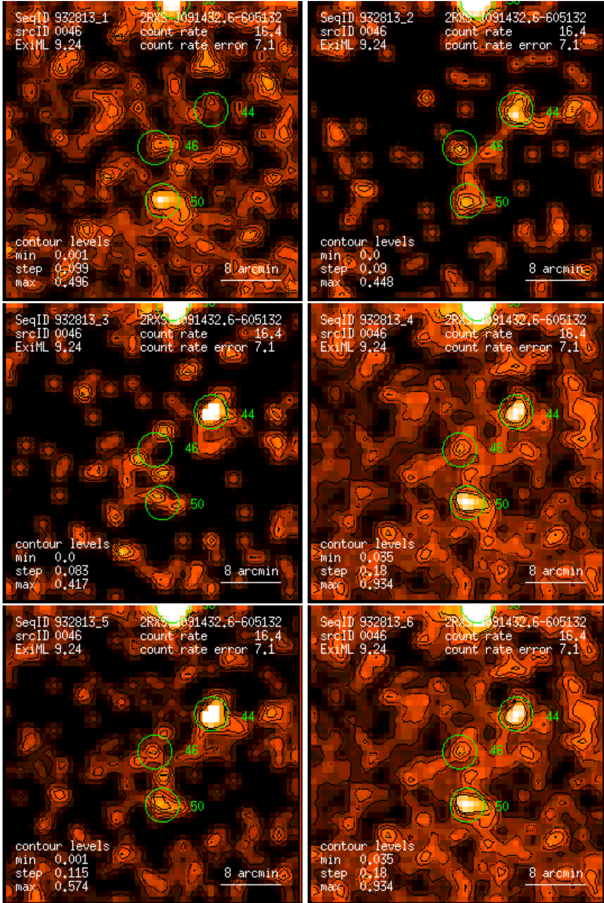
Figure 46: RASS 932813: detection 0046: band rate images, Gaussian filter: (1) PSPC channels 11 – 41, (2) 52 – 90, (3) 91 – 201, (4) 11 – 235, (5) 52 – 201, (6) 11 – 201. Broad band rates in counts/ks. Band rate contour levels in counts/ks/arcmin 2 .
