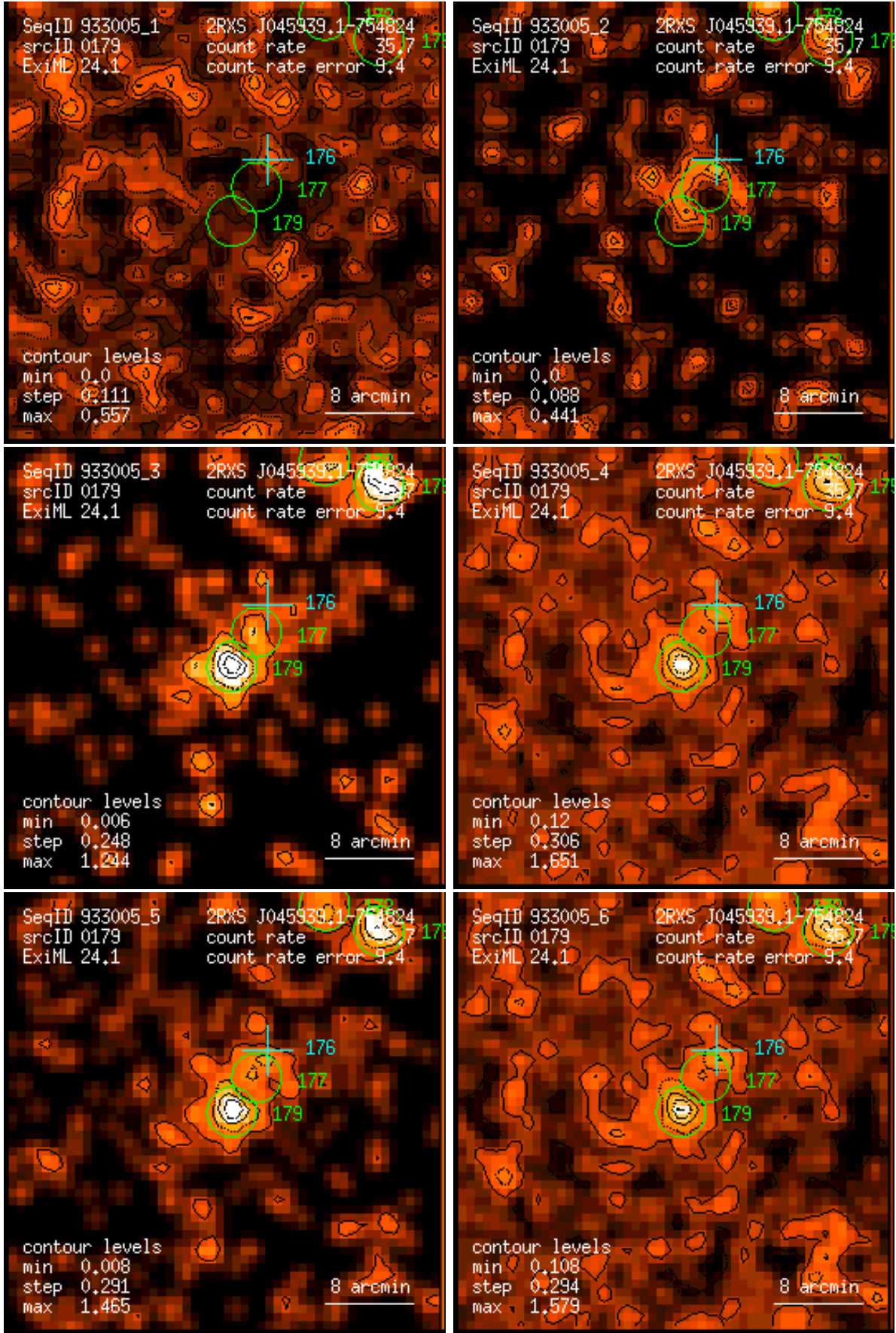
Figure 179: RASS 933005: detection 0179: band rate images, Gaussian filter: (1) PSPC channels 11 – 41, (2) 52 – 90, (3) 91 – 201, (4) 11 – 235, (5) 52 – 201, (6) 11 – 201. Broad band rates in counts/ks. Band rate contour levels in counts/ks/arcmin 2 .
