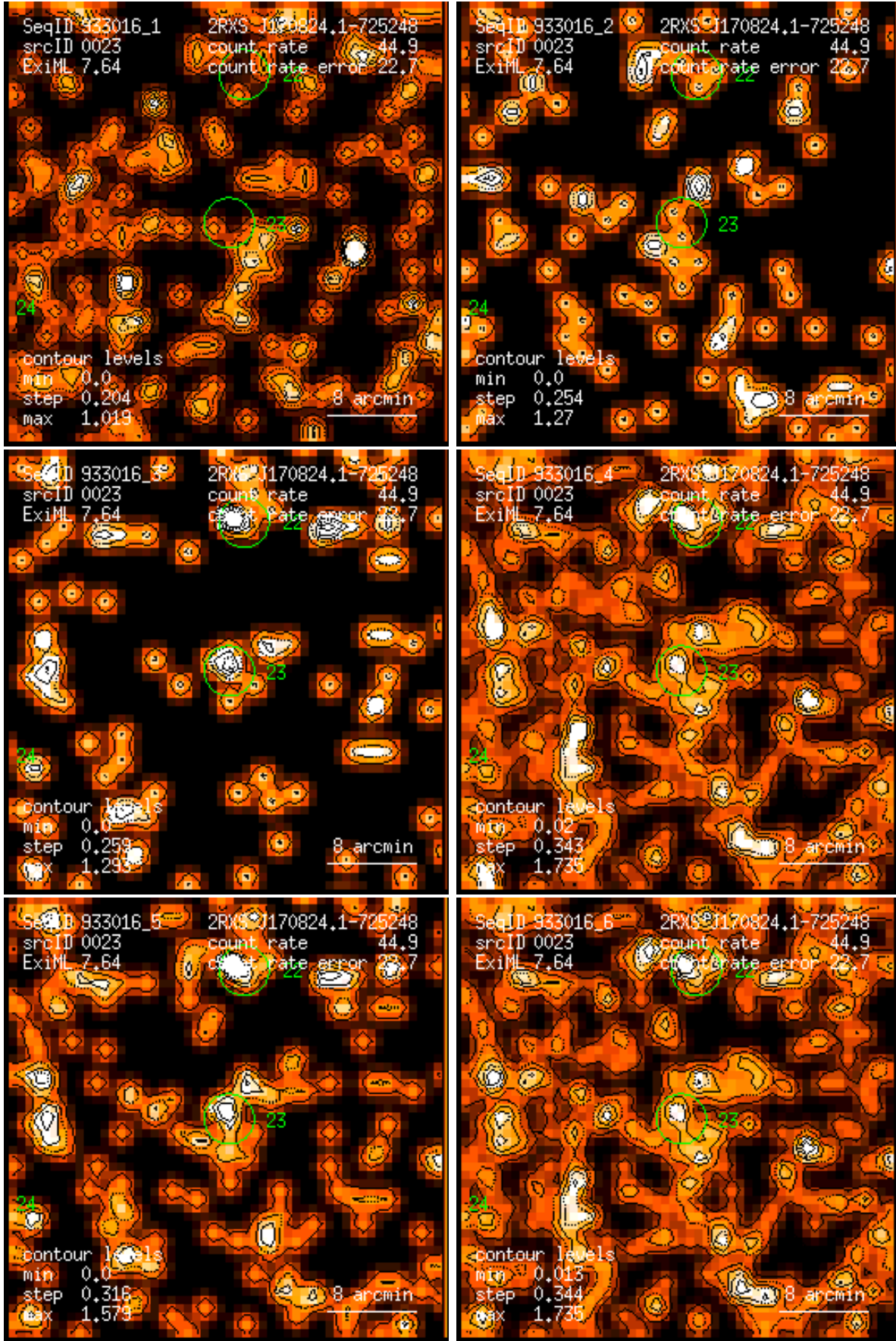
Figure 23: RASS 933016: detection 0023: band rate images, Gaussian filter: (1) PSPC channels 11 – 41, (2) 52 – 90, (3) 91 – 201, (4) 11 – 235, (5) 52 – 201, (6) 11 – 201. Broad band rates in counts/ks. Band rate contour levels in counts/ks/arcmin 2 .
